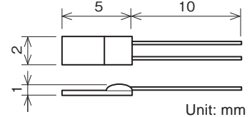
External dimensions
